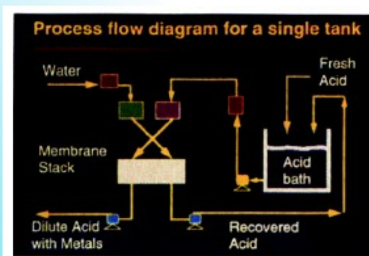
Figure 1. Acid-recycling flow schematic.
